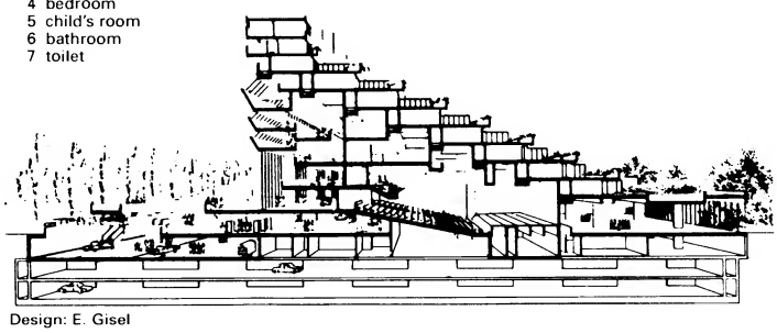
⑬ Section through a convention centre
